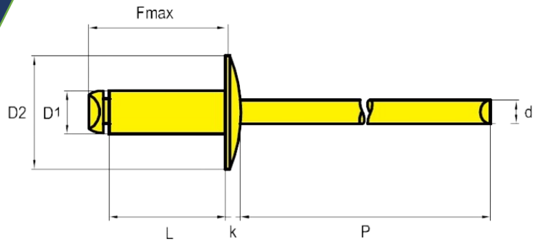
Blind Rivet Large Flange Dome Head
