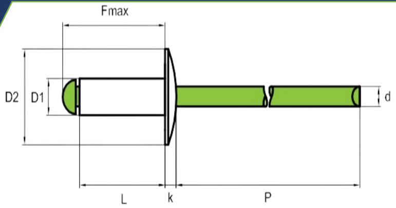
Blind Rivet Large Flange Dome Head
