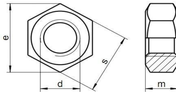
Hex Nut ASME B 18.2.2 (UNC Series)
