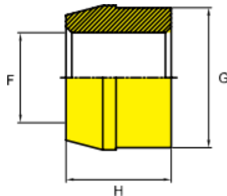
Collar Nut for Pin Standard Brazier Head
