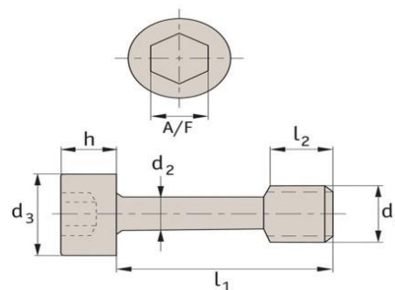
CAPTIVE SCREW ALLEN CAP (Self Colour)
